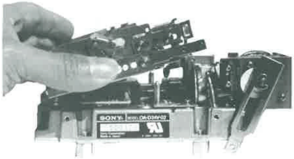
Figure 13-20 Carrier mechanism removal.
