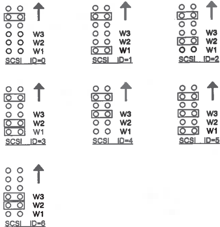
Figure 14-25 SCSI address pins—configuration details.
