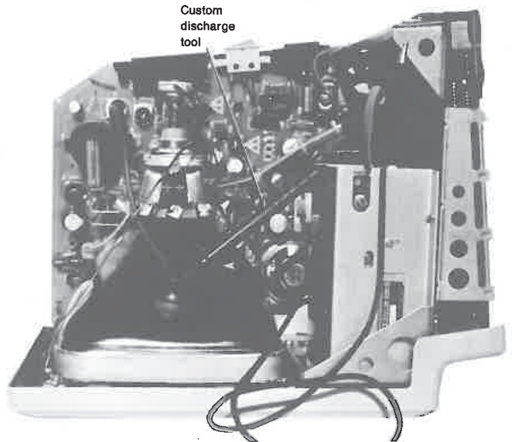
Figure 1-15 An easy-to-make custom discharge tool.
