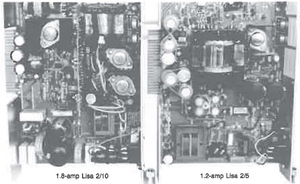
Figure 13-7 Lisa/Mac XL power supplies—internal views. 1.8-A Lisa 2/10 to Mac XL power supply is shown on the left. 1.2-A Lisa 2/5 power supply is shown on the right. Note the three power transistors and the extra large filter caps in the Lisa 2/10 to Mac XL model.
