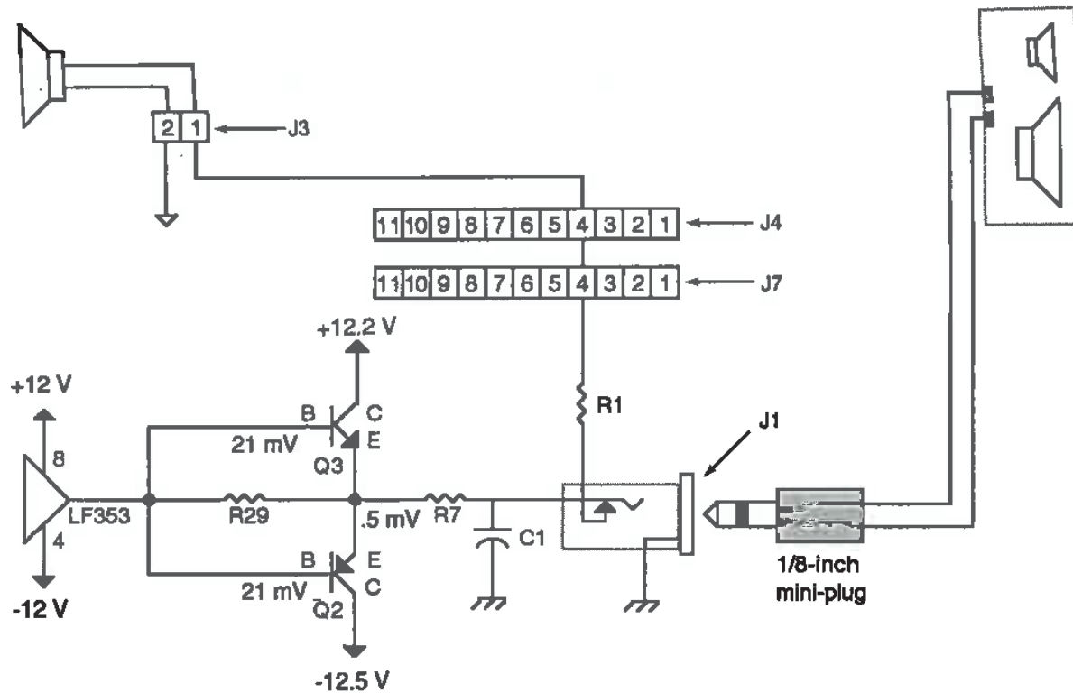
Figure 8-1 Macintosh audio circuit, 820-0086-C logic board.
