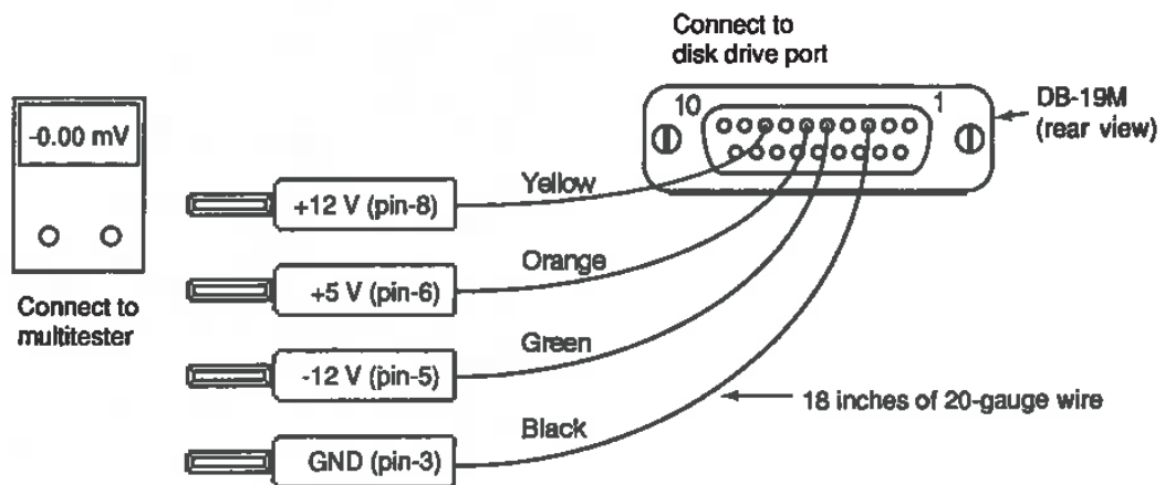
Figure 14-4 Voltage checking adapter for 128K to Mac SE. Not for Lisas and Mac XL's.
