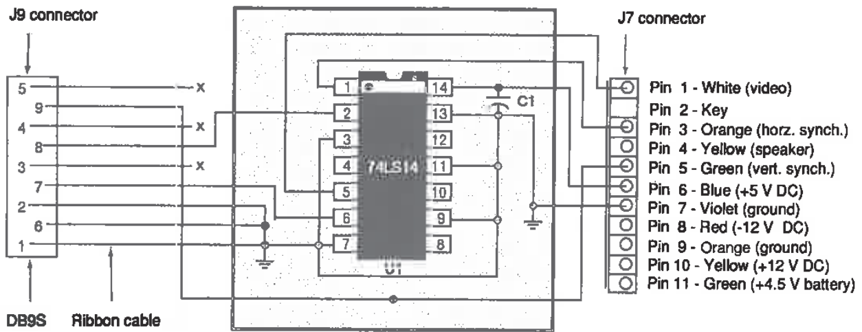
Figure 9-6 Wiring diagram for TTL video adapter.
