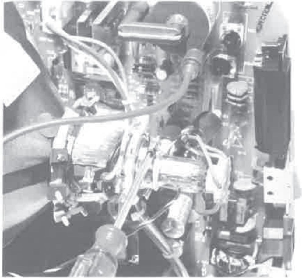
Figure 9-2 Yoke retaining screw—removal details.
