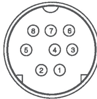
Rear View (solder side)
