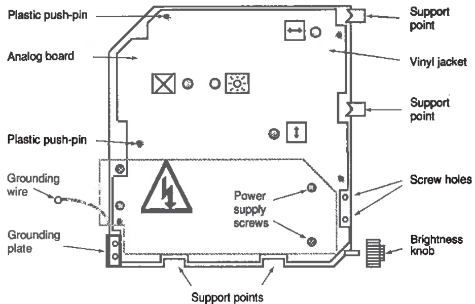
Figure 14-2 Mac SE— analog board mounting details.
