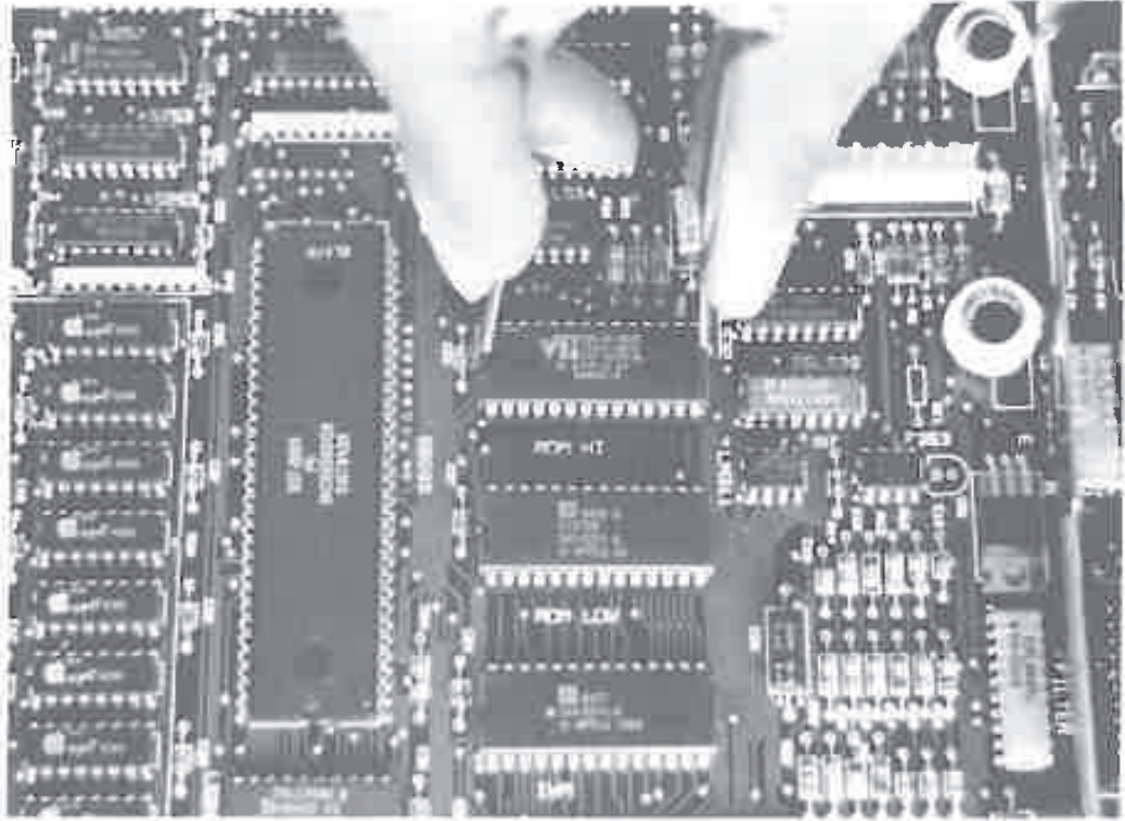
Figure 10-10 Remove the old ROMs with an IC-puller.
