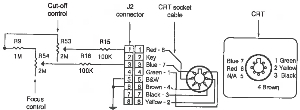
Figure 4-16 When the focus control has no effect, or an intermittent effect, it's usually due to: 1. Burned resistors in the focus circuit 2. A loose or corroded CRT socket cable 3. Tarnish on the CRT pins.
