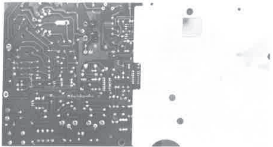
Figure 6-4 Compound problems. Physical evidence of T1 having failed while the computer was unattended.
