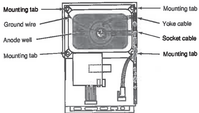
Figure 9-4 CRT mounting details.
