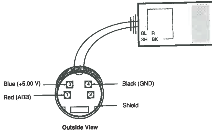
Figure 14-19 Pinouts for the ADB mouse connector.
