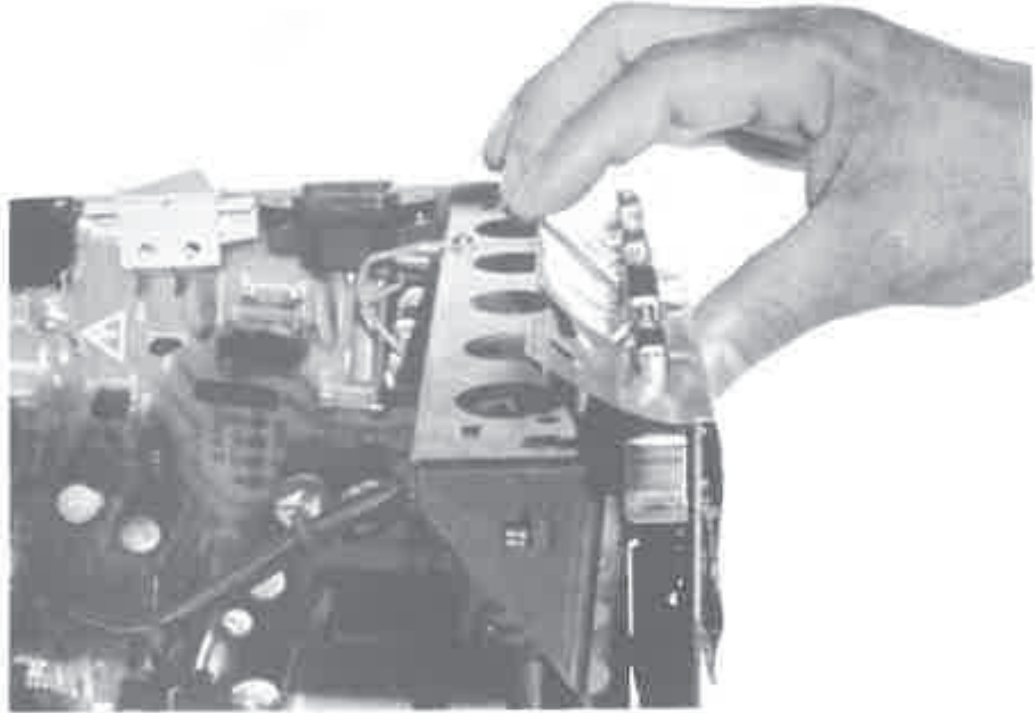
Figure 1-9 The RFI shield is a 9-inch long, L-shaped piece of aluminum-colored material that fits over the I/O connectors on the logic board.
