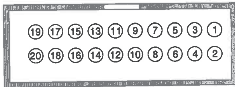
Figure 10-15 Disk drive socket header pinouts.
