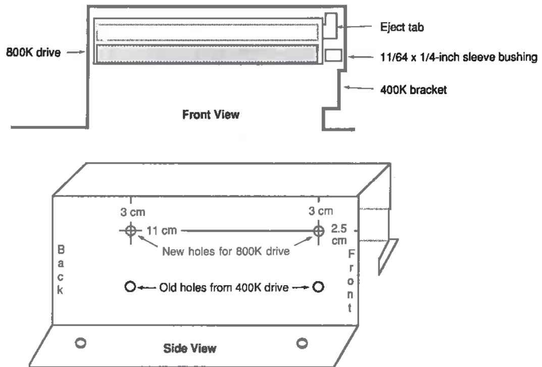
Figure 10-14 400K disk drive bracket modifications.
