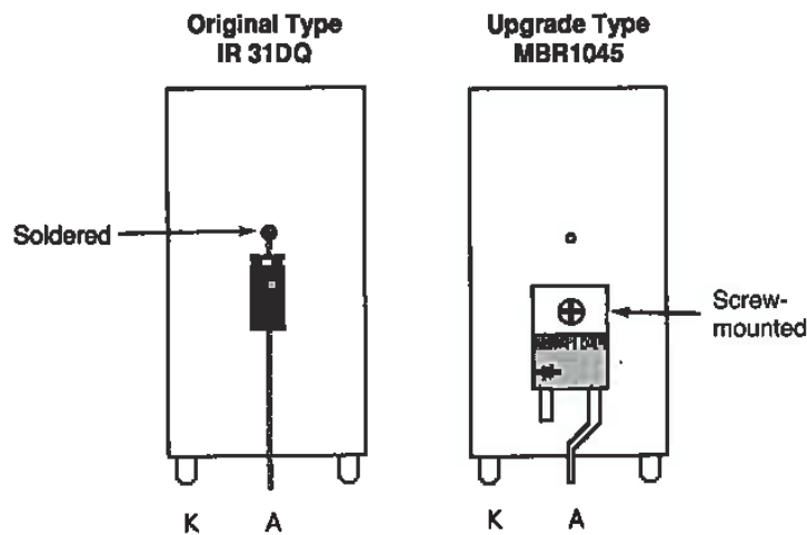
Figure 7-1 Mounting details for CR20 and CR21 upgrades.
