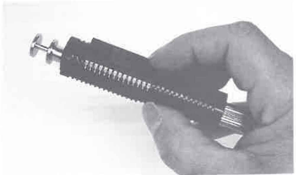
Figure 10-12 Straighten bent pins with a pin-straightener.
