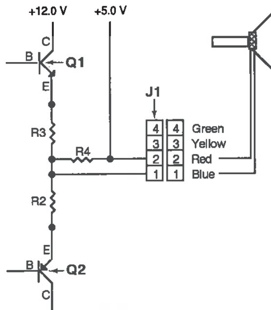
Figure 5-21 The schematic relationship between Q1, Q2 (International Q4), R2, and R3.
