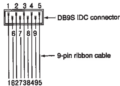
Figure 9-7 Numbering details for DB9S IDC connector.
