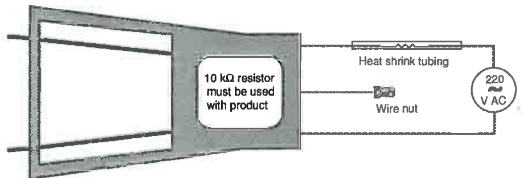
Figure 7-8 Wiring details for 220-V AC 50-Hz piezoelectric fan. One of the outer fan wires goes through a 10-k \Omega resistor to the AC line. The other outer fan wire goes directly to the AC line. The inner fan wire is tied off.
