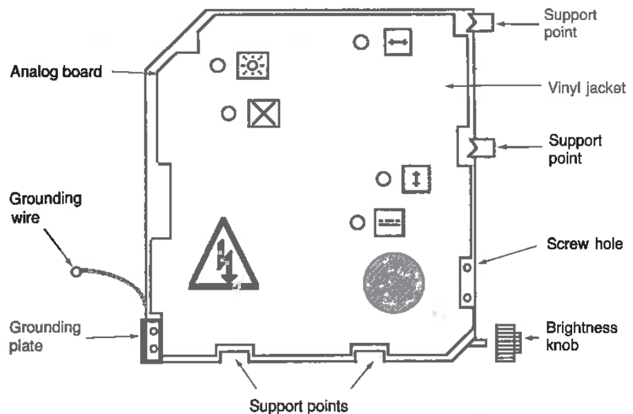
Figure 7-5 Analog board mounting details.
