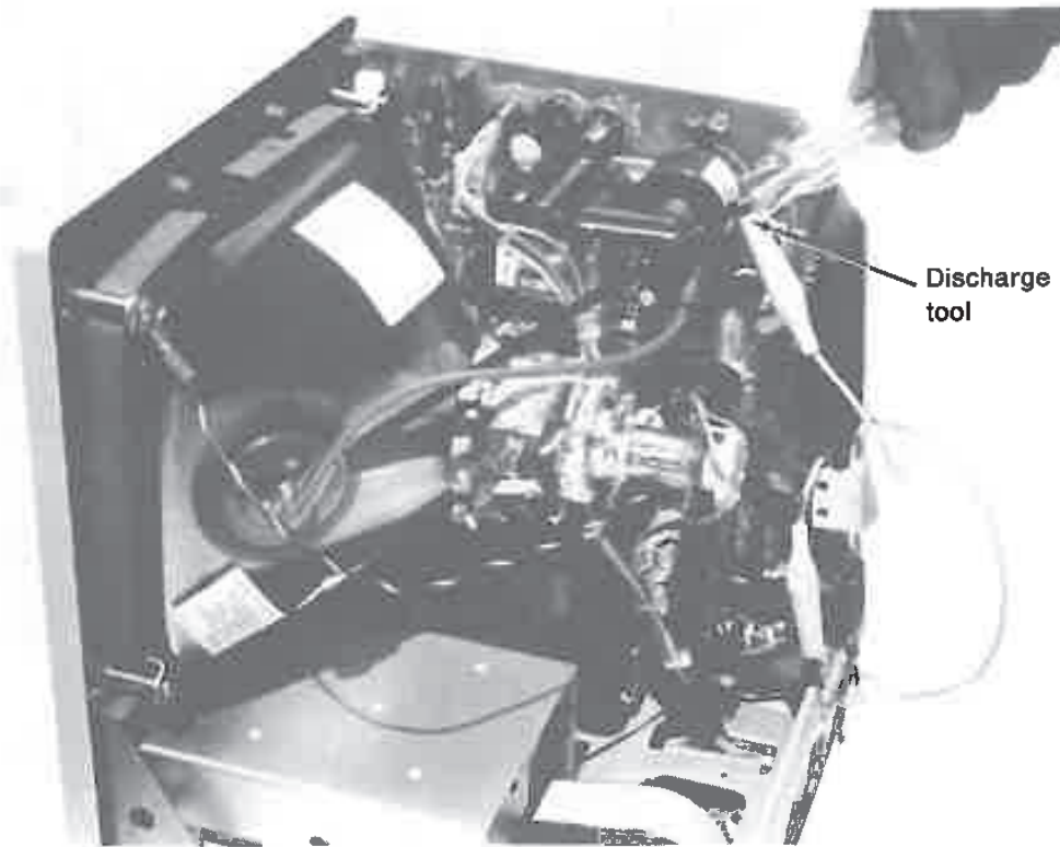
Figure 1-13 You can discharge the picture tube with an insulated long-handled screwdriver, a green clip lead, and a 10-megohm resistor.
