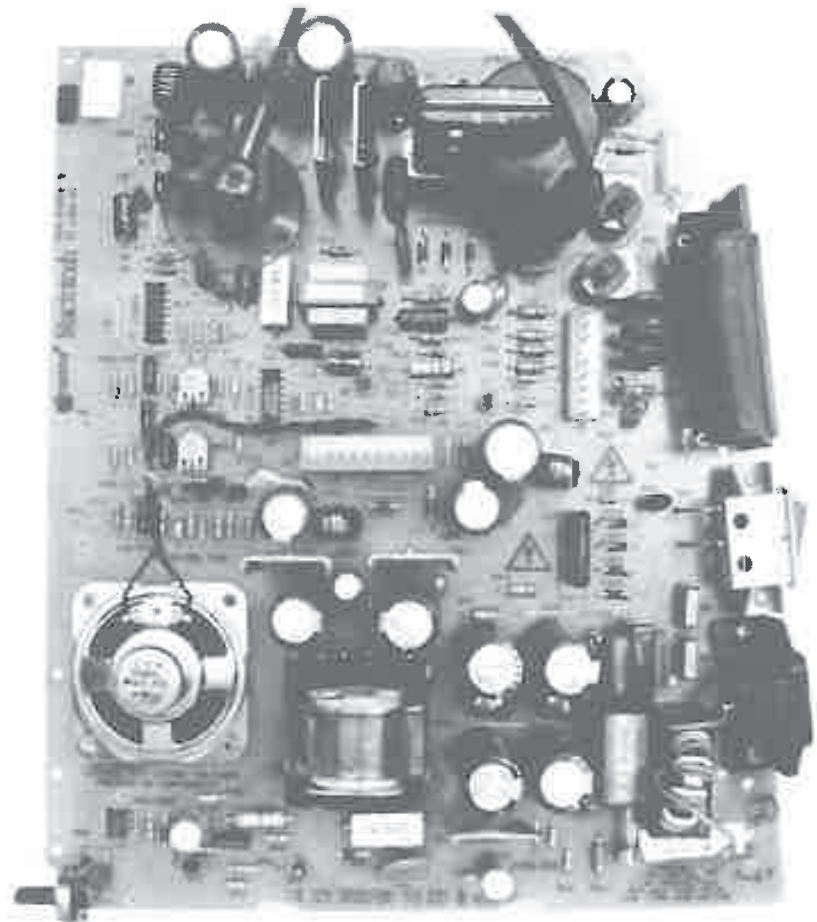
Figure 4-2 The International version of the 128K to Mac Plus analog board has a convertible 120/240-V power supply.
