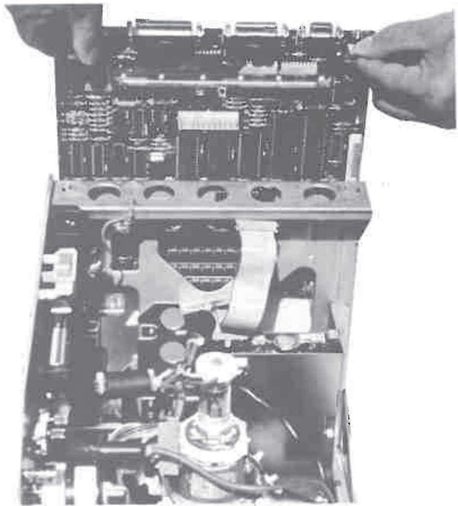
Figure 10-1 Logic board removal.
