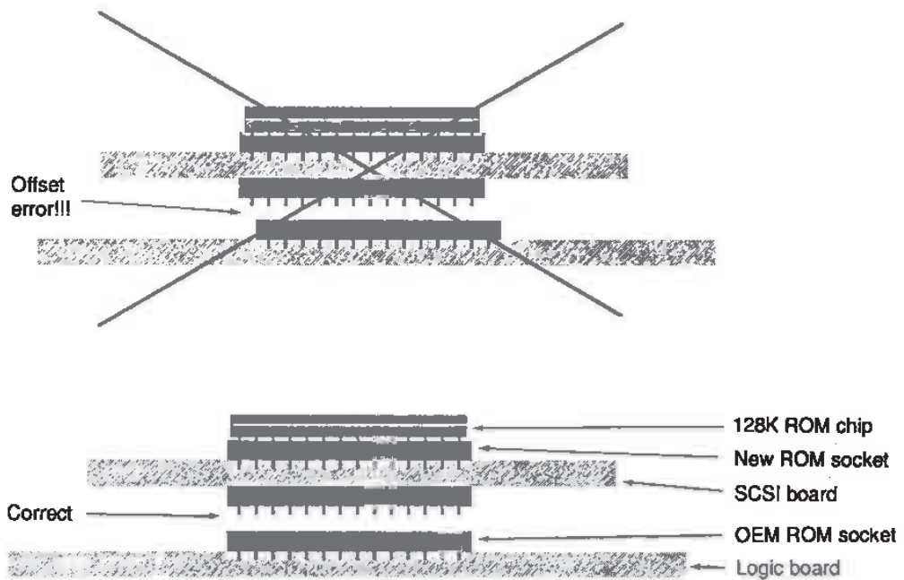
Figure 10-20 Plug-in SCSI board alignment details.
