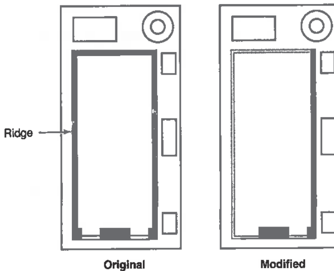
Figure 10-19 Battery compartment modification details.
