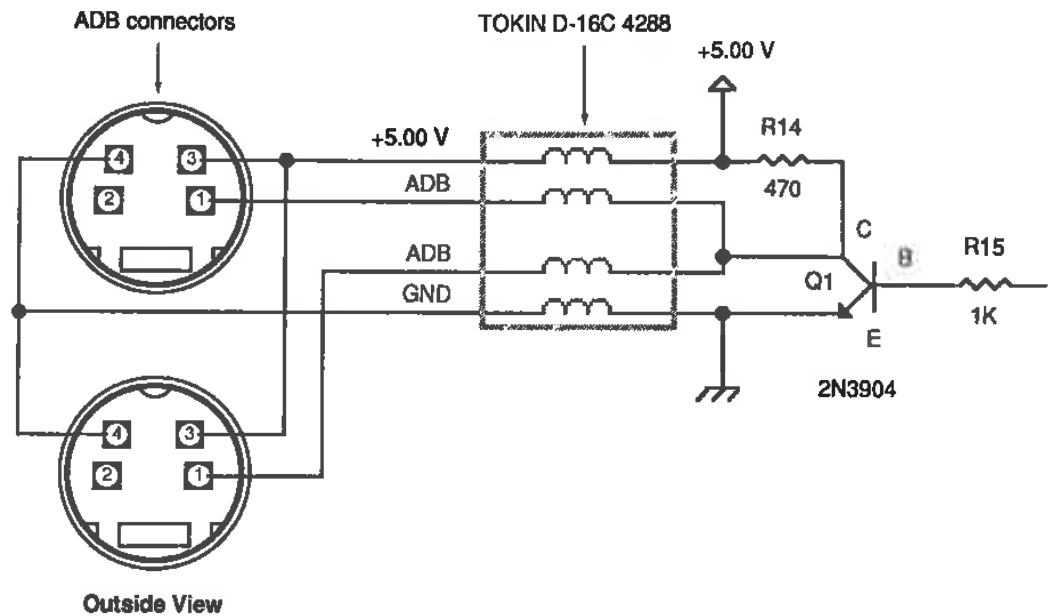
Figure 14-20 ADB schematic.
