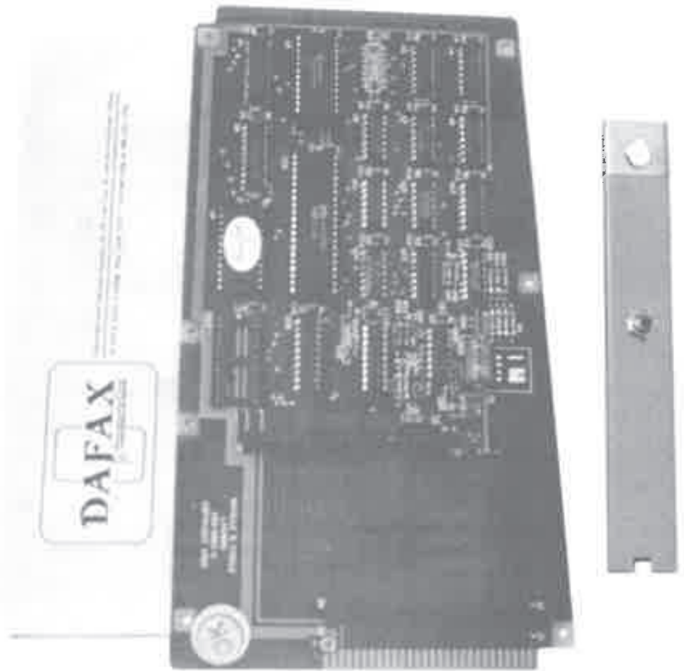
Figure 13-30 Multivoice sound card for the Lisa/Mac XL.
