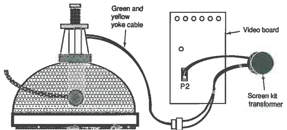
Figure 13-32 XL screen kit wiring details.
