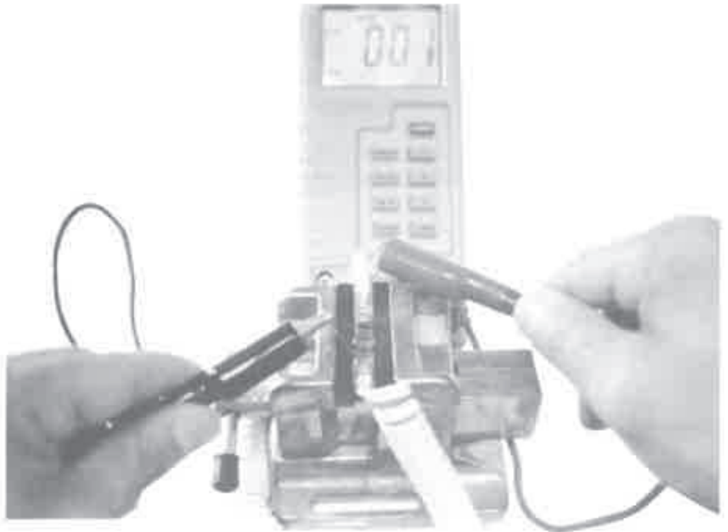
Figure 11-21 Checking the cable for continuity.
