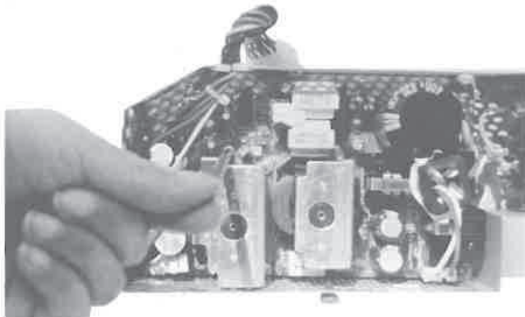
Figure 14-7 Mac SE internal power supply adjustment.
