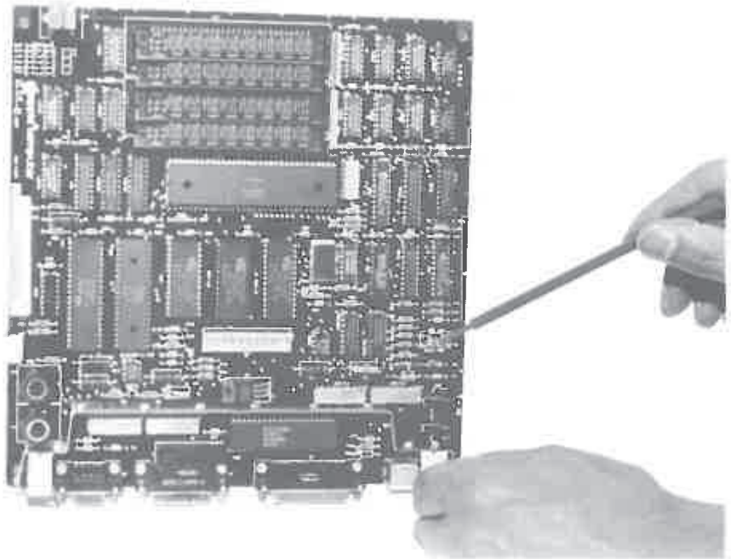
Figure 10-23 Location of Mac Plus memory size resistors.
