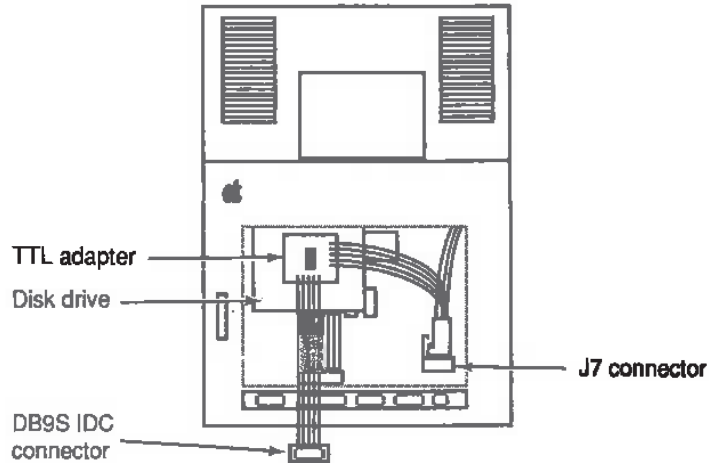
Figure 9-8 TTL video adapter—mounting detail for 128K to Mac Plus.
