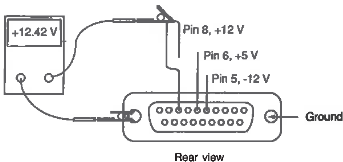
Figure 2-19 Measuring voltages at the disk drive connector.
