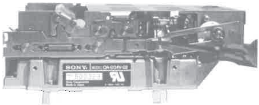
Figure 13-18 C-ring removal.
