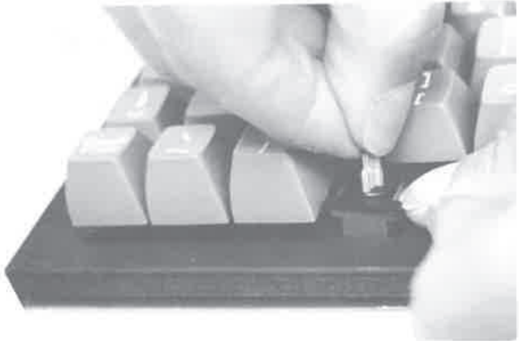
Figure 11-13 The new switch snaps into place.
