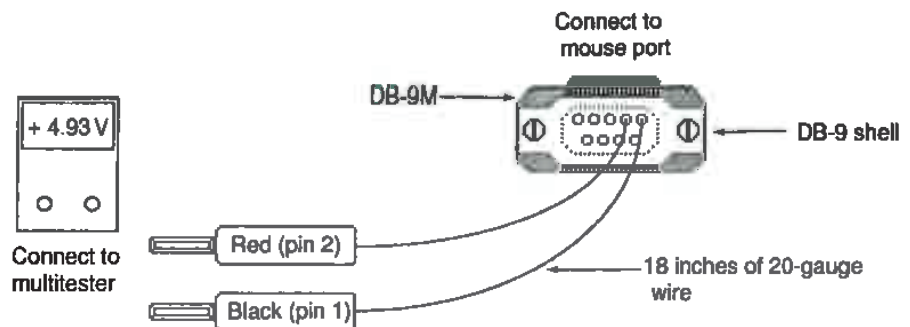
Figure 2-20 Voltage checking adapter for 128K to Mac Plus, Lisas, and Mac XL's. Not for Mac SE.
