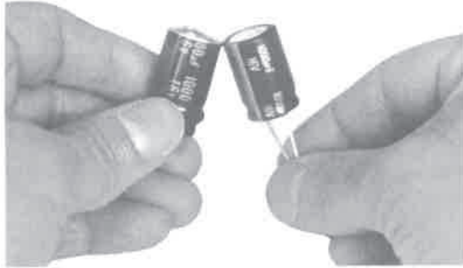
Figure 6-5 Shorted capacitor. Sometimes, electrolytic failure is obvious.
